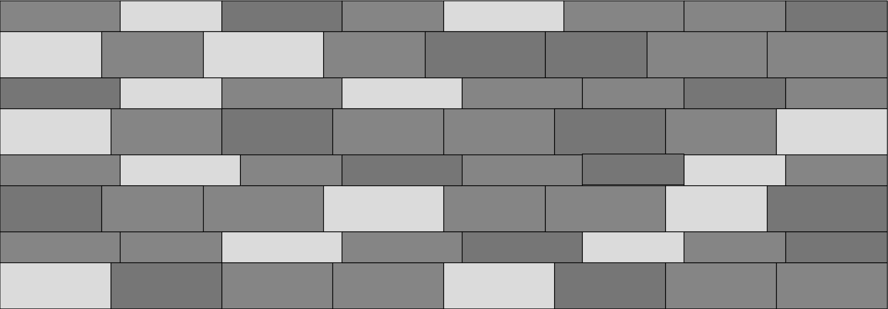
650X250X80 550X250X80 550X167X80 650X167X80 600X250X80
